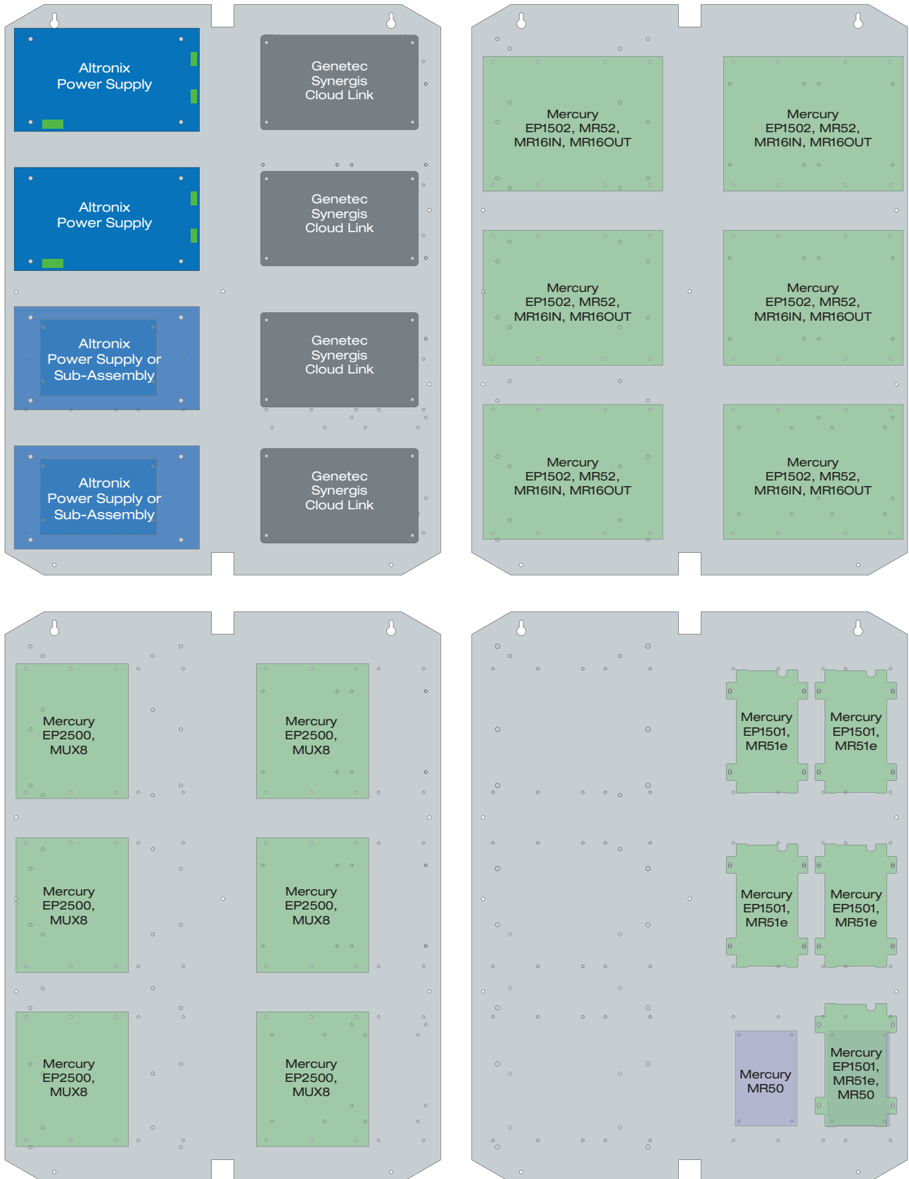
Trove2M2 Interior Backplane - Optional Mounting Configurations
